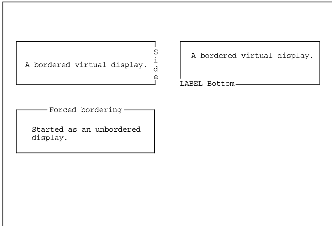
Figure SMG-31 Output Generated by Program Calling SMG$LABEL_BORDER
