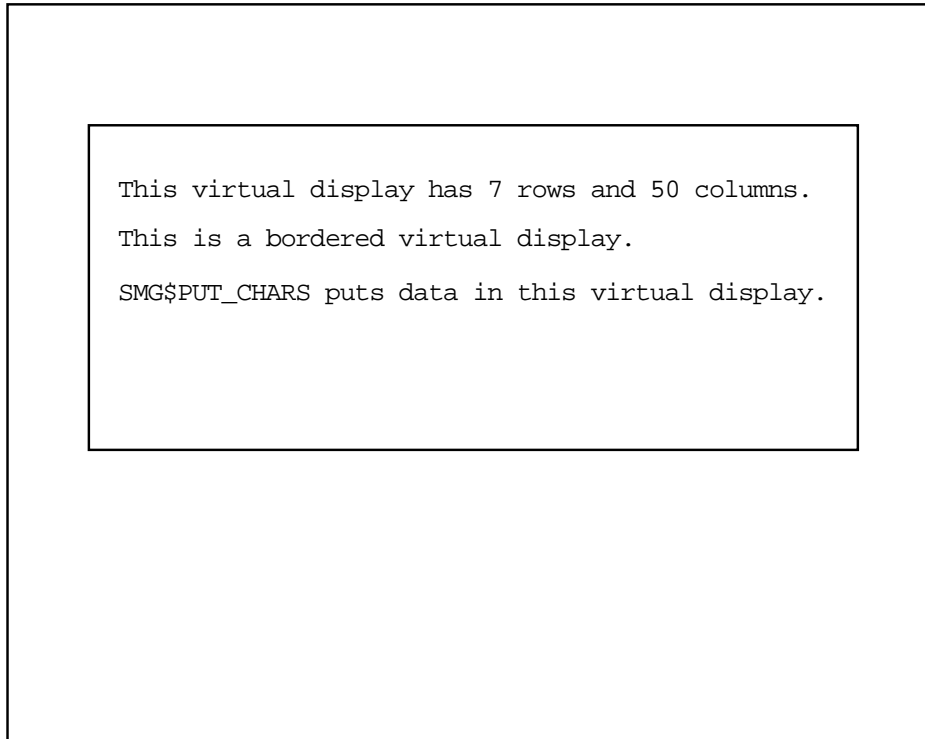
Figure SMG-22 Initial Output of Fortran Program Calling SMG$ERASE_DISPLAY
