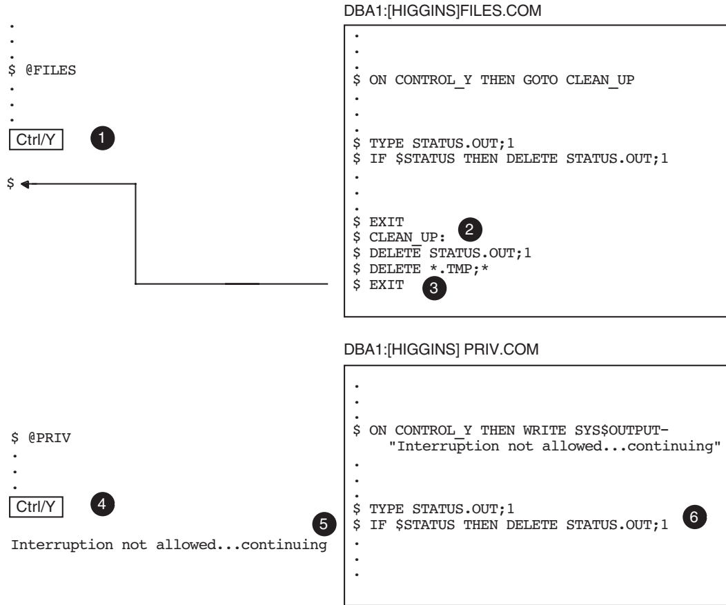
Figure 13–2 Flow of Execution Following Ctrl/Y Action
